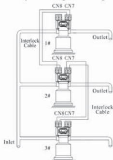
Figure 3-12 Interlock system
