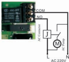
Figure 3-8 Wiring of Booster Pump on Inlet
