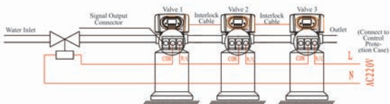
Figure 3-4 Wiring of Solenoid Valve in Inlet
