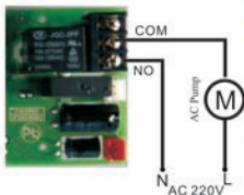
Figure 3-7 Wiring of Booster Pump on Inlet
